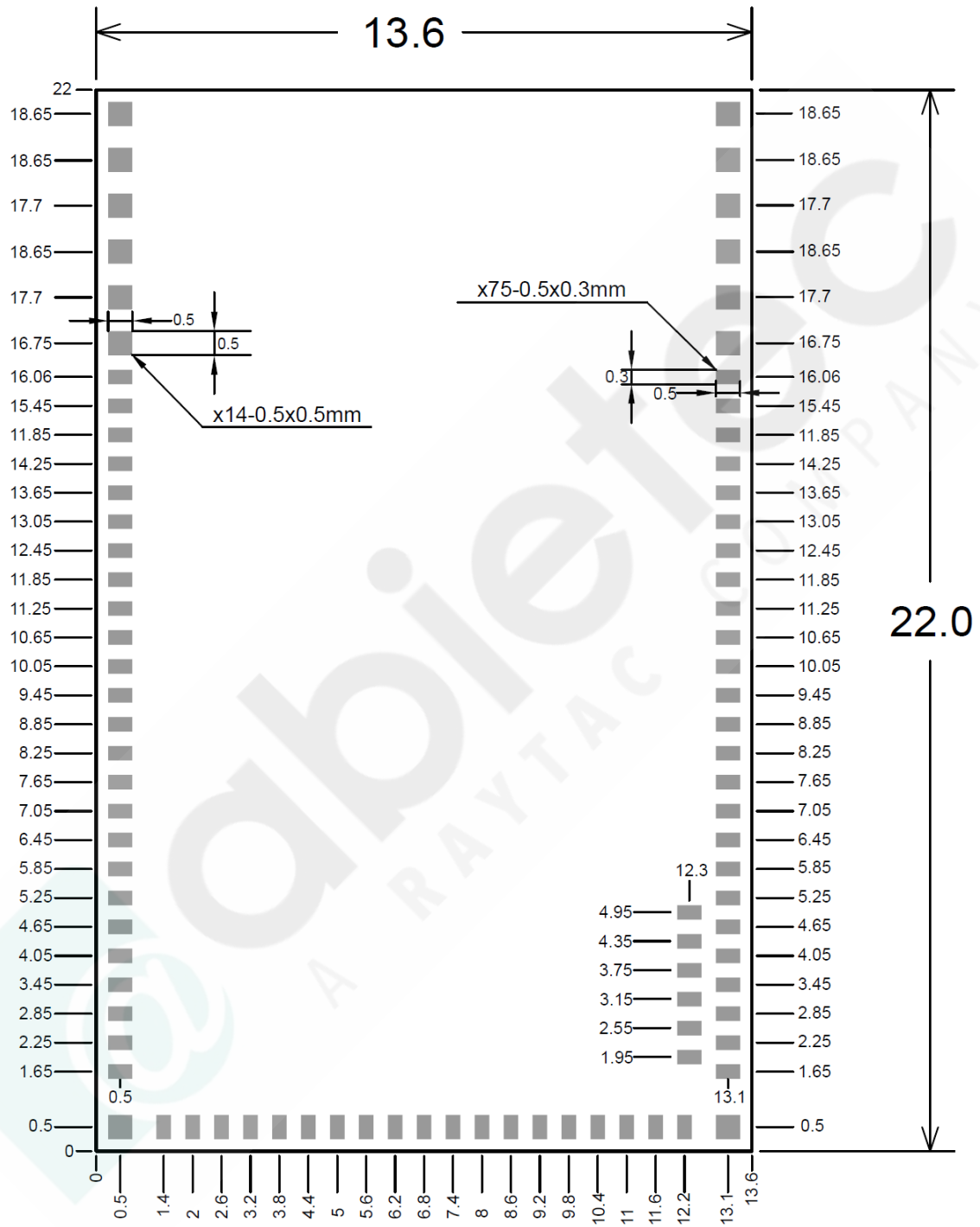
Top View (Unit: mm)
