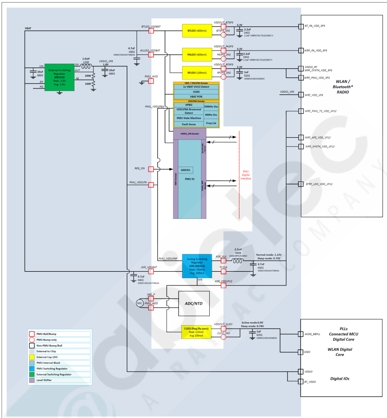
Figure 1 Typical power topology
