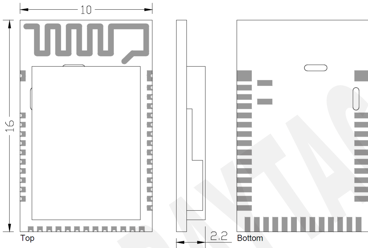
PCB Size (in mm)
